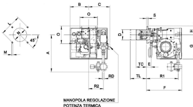
Model GAS 1/C - GAS 2/C / Modello GAS 1/C - GAS 2/C
