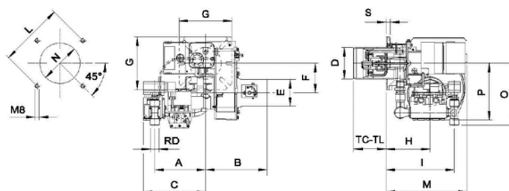
Model GAS X0 THLS / Modello GAS X0 THLS
