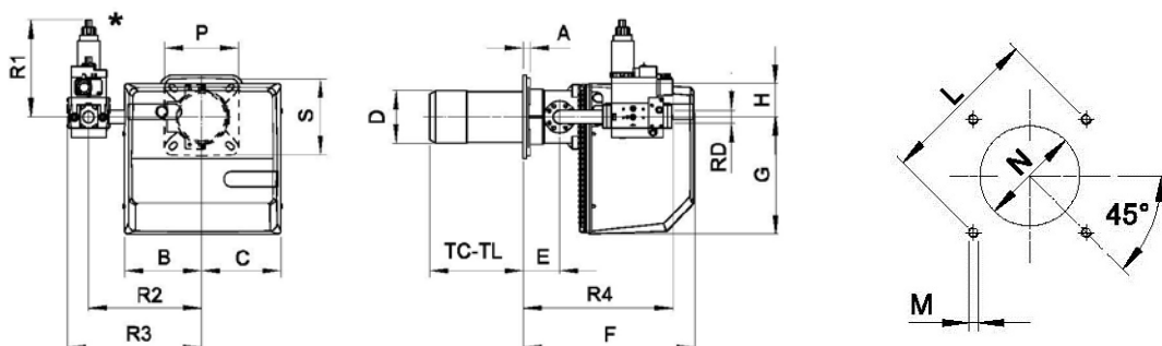
Model GAS X5/2 / Modello GAS X5/2
